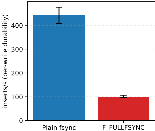
Durability tax: throughput
