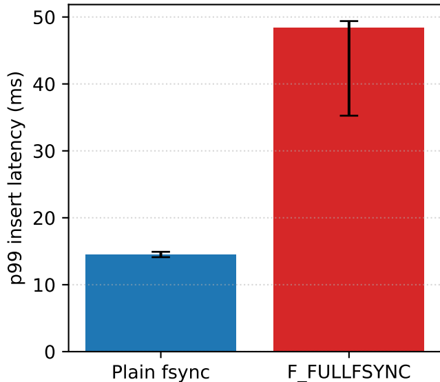
Durability tax: tail latency
