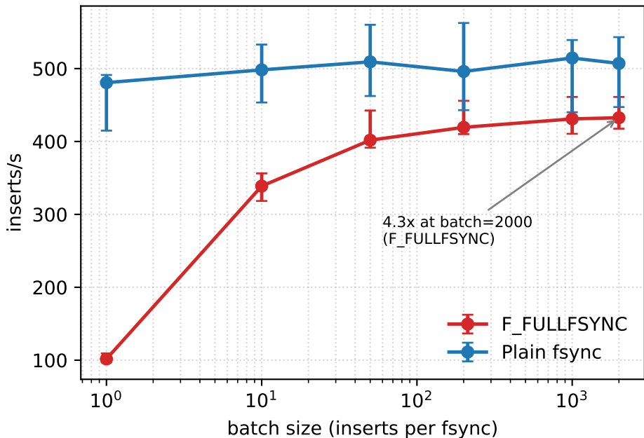
Group commit: throughput vs. batch size
