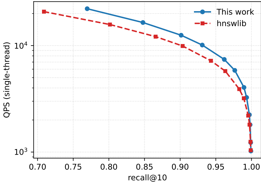
SIFT1M: recall vs. throughput (up-and-right is better)
