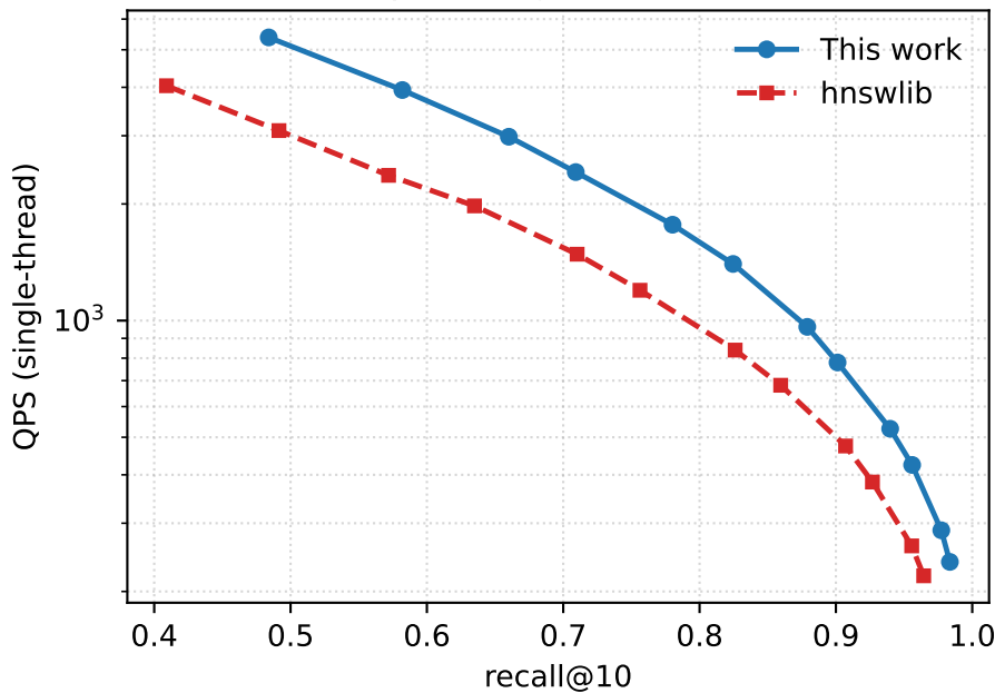
GIST1M: recall vs. throughput (up-and-right is better)
