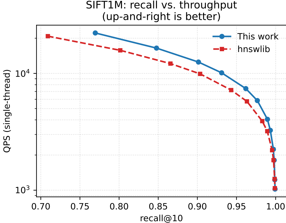
Figure 3: SIFT1M recall-QPS Pareto front (single-thread, Apple M4 Pro). Our index (solid) tracks hnsplib (dashed) across the operating range: over matched it averages +1.8 recall points (deterministic) at a mean 1.02\times QPS (single-run, within timing noise), i.e. the two are Pareto-equivalent. Up-and-to-the-right is better.
