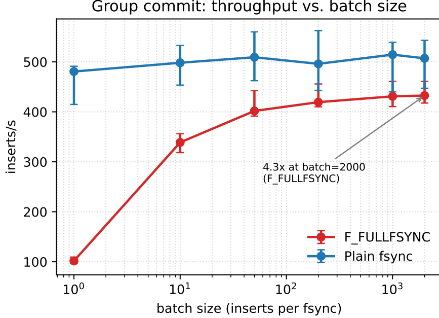
Figure 1: Group commit throughput vs. batch size (Apple M4 Pro, d=128 ; median of 7 trials, min-max whiskers). Under F_FULLFSYNC the curve rises from 102 to 433 inserts/s (4.3 \times ) as the flush is amortized; under plain fsync it is flat, because the page-cache “flush” costs almost nothing. The two converge at large batches: once the flush leaves the critical path, HNSW graph insertion is the bound.
