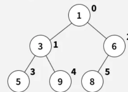
Representation of a Binary Heap
