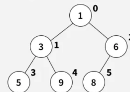
Representation of a Binary Heap
