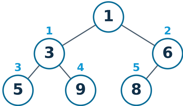
Baum 0
