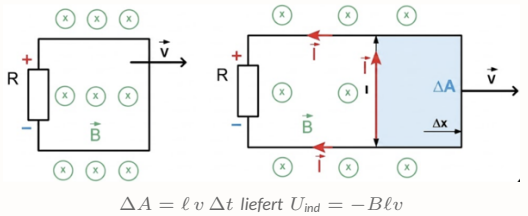
\Delta A = \ell v \Delta t liefert U_{\text{ind}} = -B \ell v
