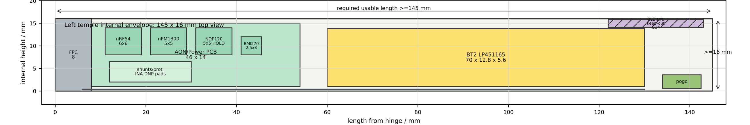
Left temple top view - AON/power + battery
