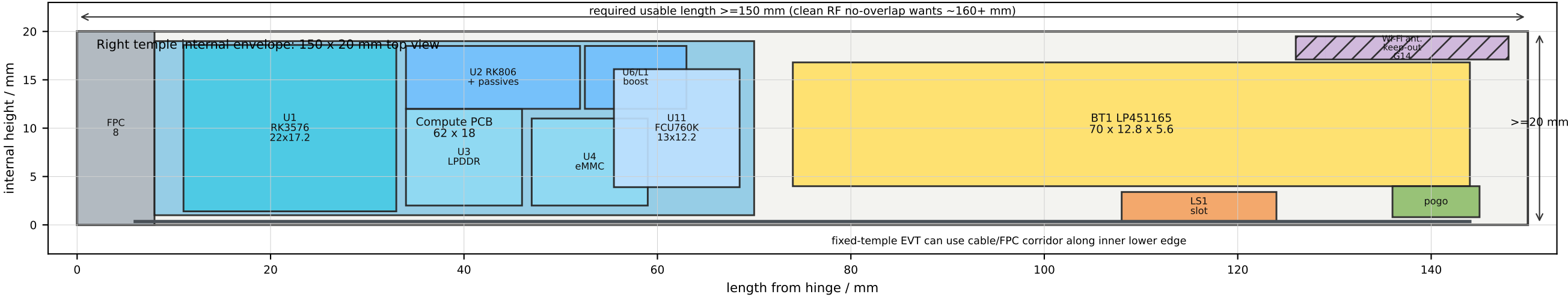
Right temple top view - compute + Wi-Fi + battery
