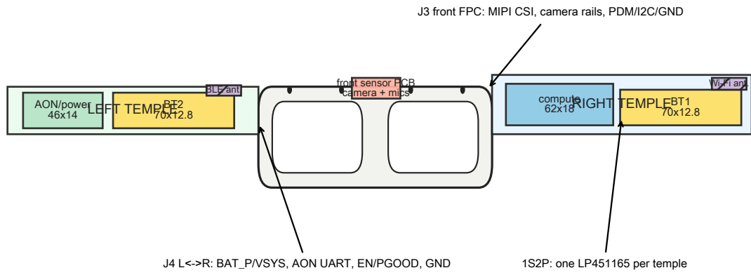
1 Whole glasses top view
