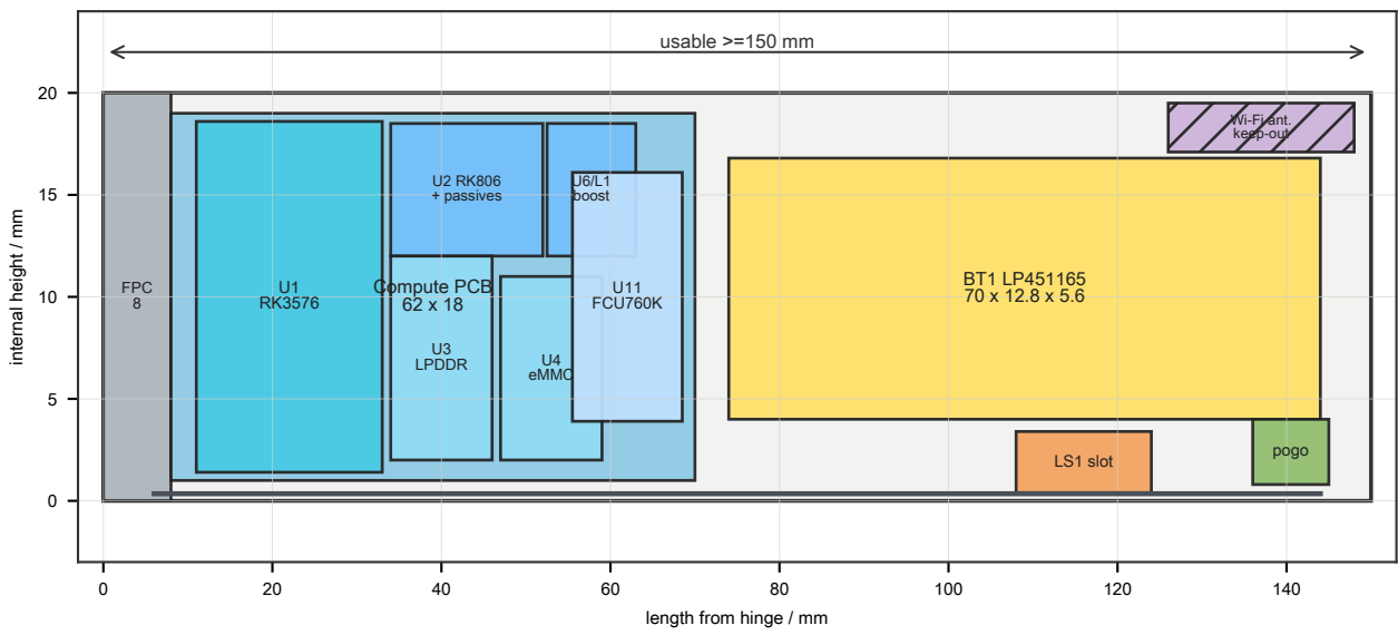
10 Right temple top view
