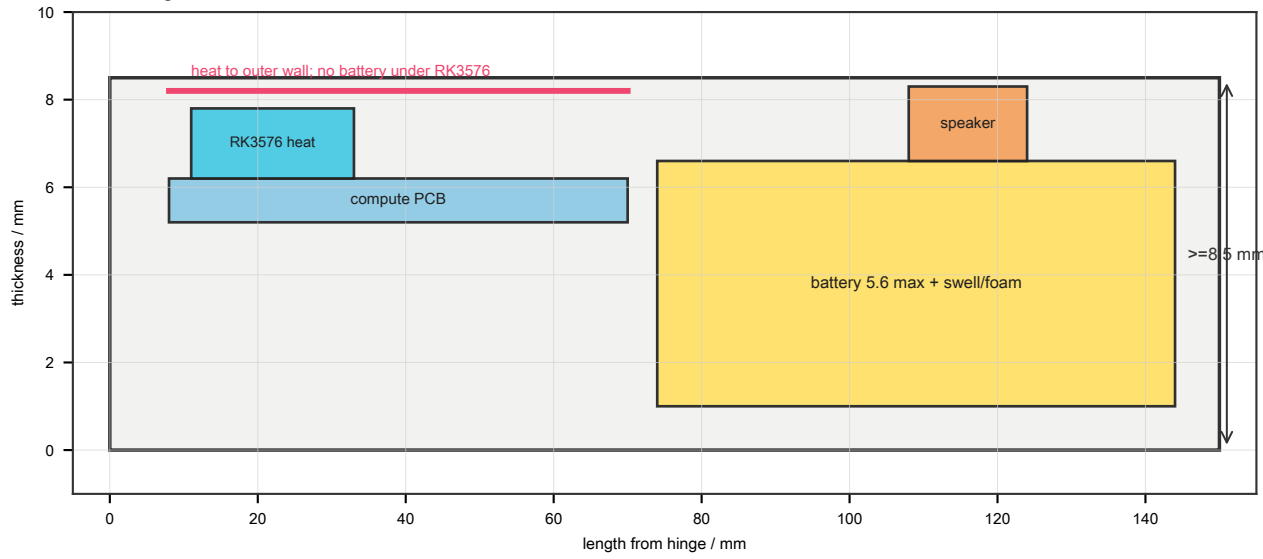
2 Whole glasses side view
