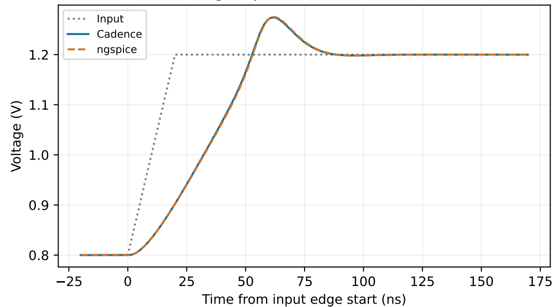
Rising step: 74.10 mV overshoot
