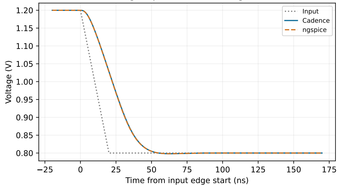
Falling step: 40.92 ns settling (1%)
