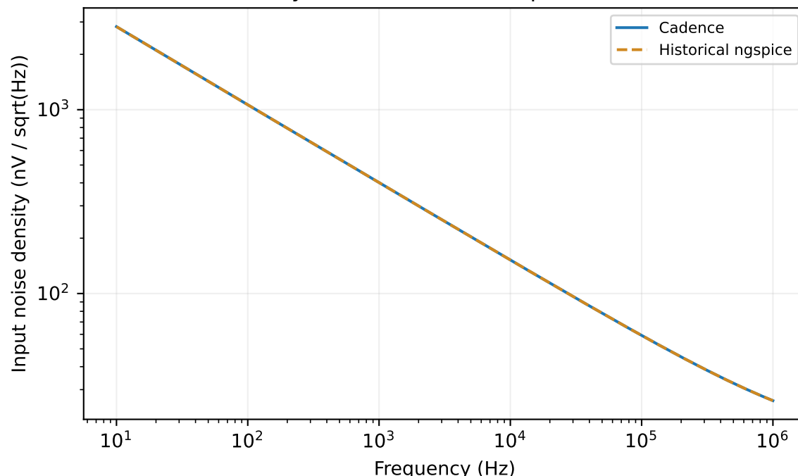
Stationary noise: 401.15 nV/sqrt(Hz) at 1 kHz
