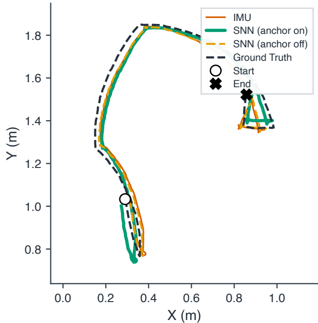
B Representative trial (ATE \approx mean)
