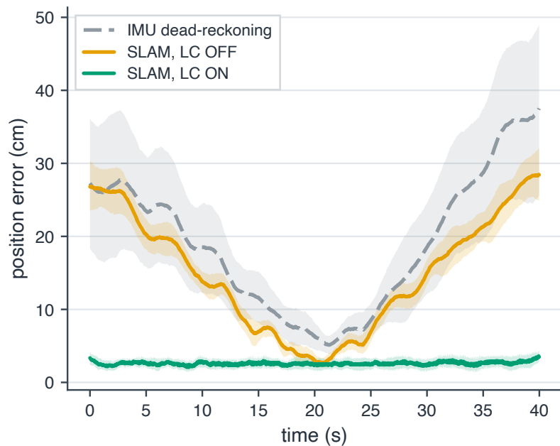
B Error vs time (mean, 95% CI band)
