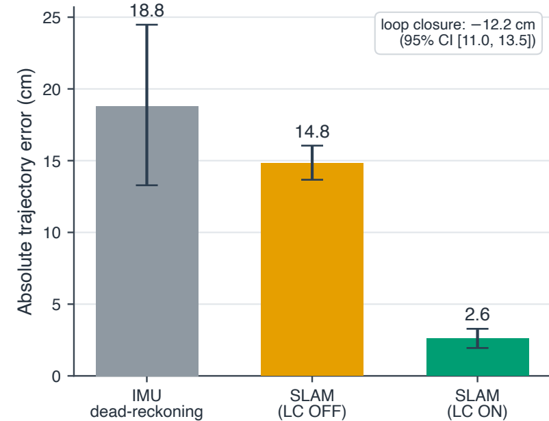
A ATE on revisit-rich circuit (n=12)
