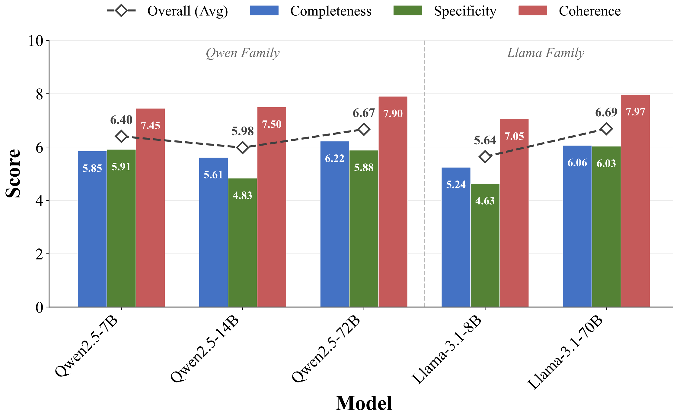
(a) Skeleton Quality Scores by Model
