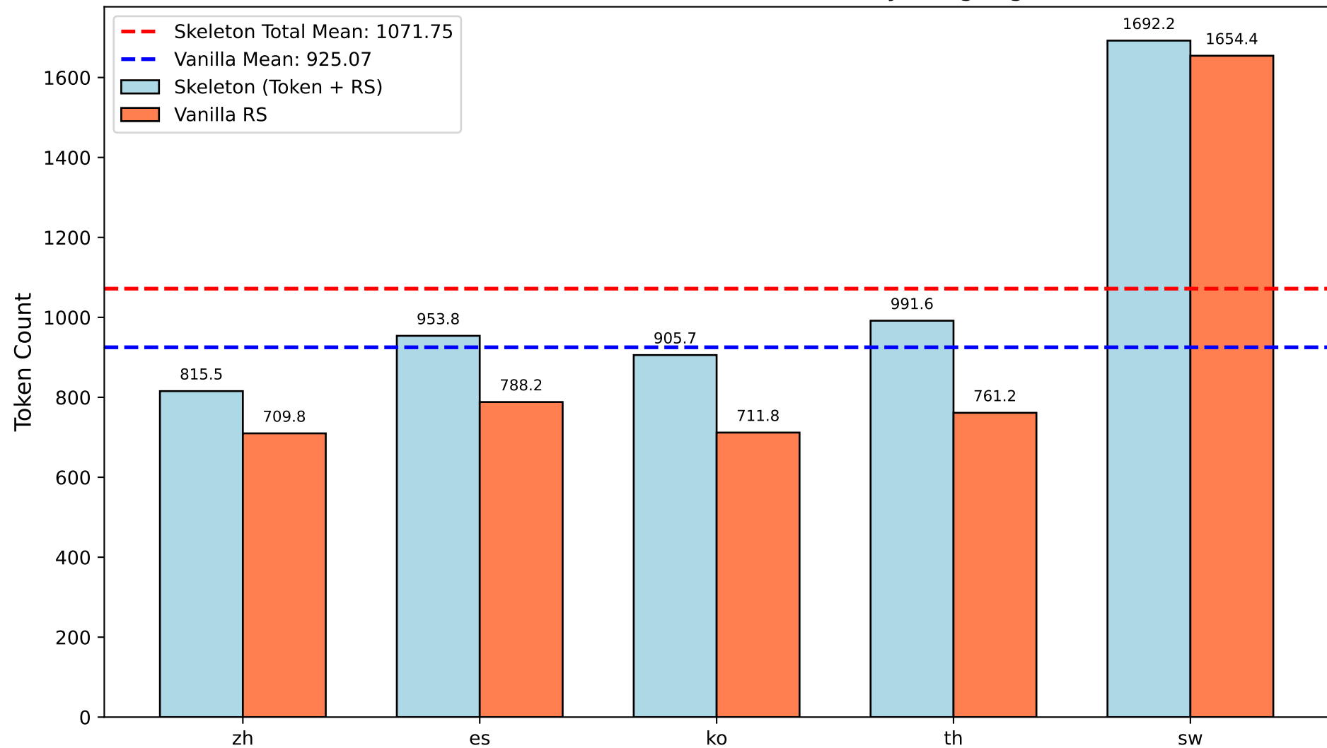
Skeleton (Token + RS) vs Vanilla RS by Language
