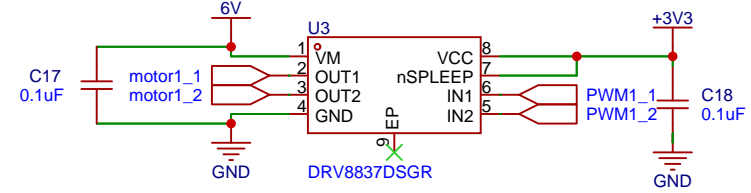
DC Driver
