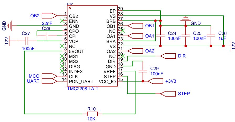
Stepper Driver
