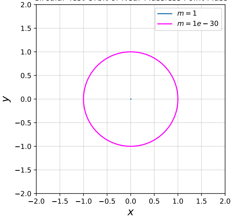
Circular Test Orbit of Near Massless Point Mass
