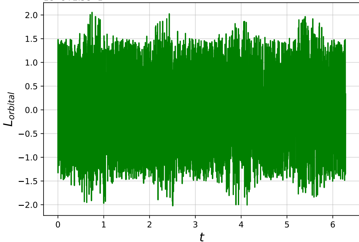
Orbital Angular Momentum vs. Time of M_1=0.5 , M_2=0.5 Binary 1e-8+2.5e-1
