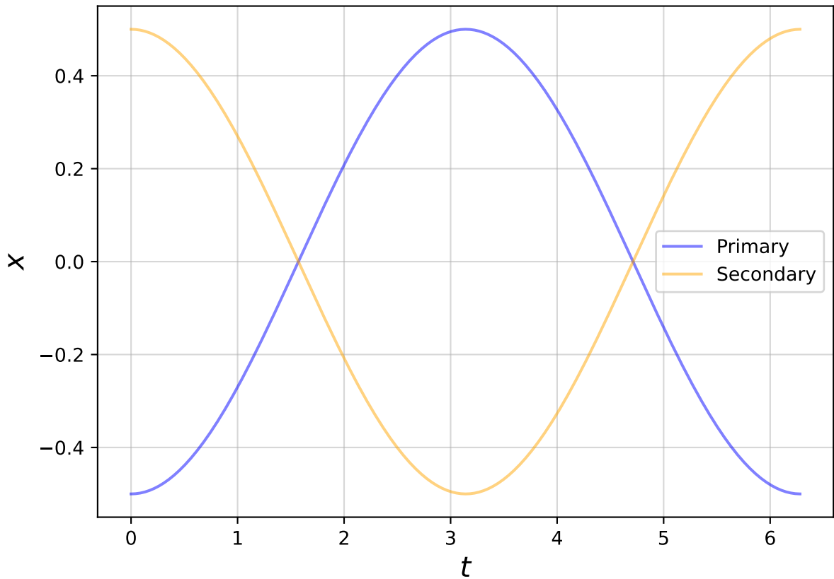
x Position vs. Time of M_1=0.5 , M_2=0.5 Binary
