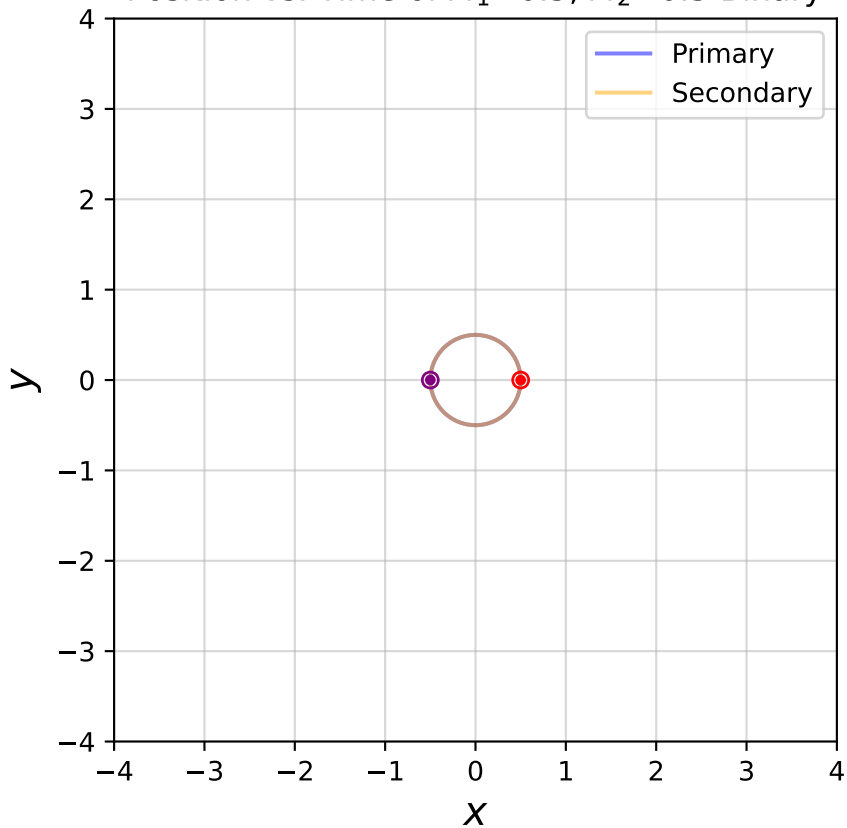
Position vs. Time of M_1=0.5 , M_2=0.5 Binary
