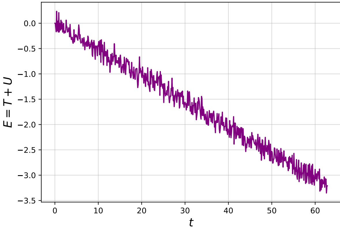
Energy vs. Time of M_1=0.5 , M_2=0.5 Binary
