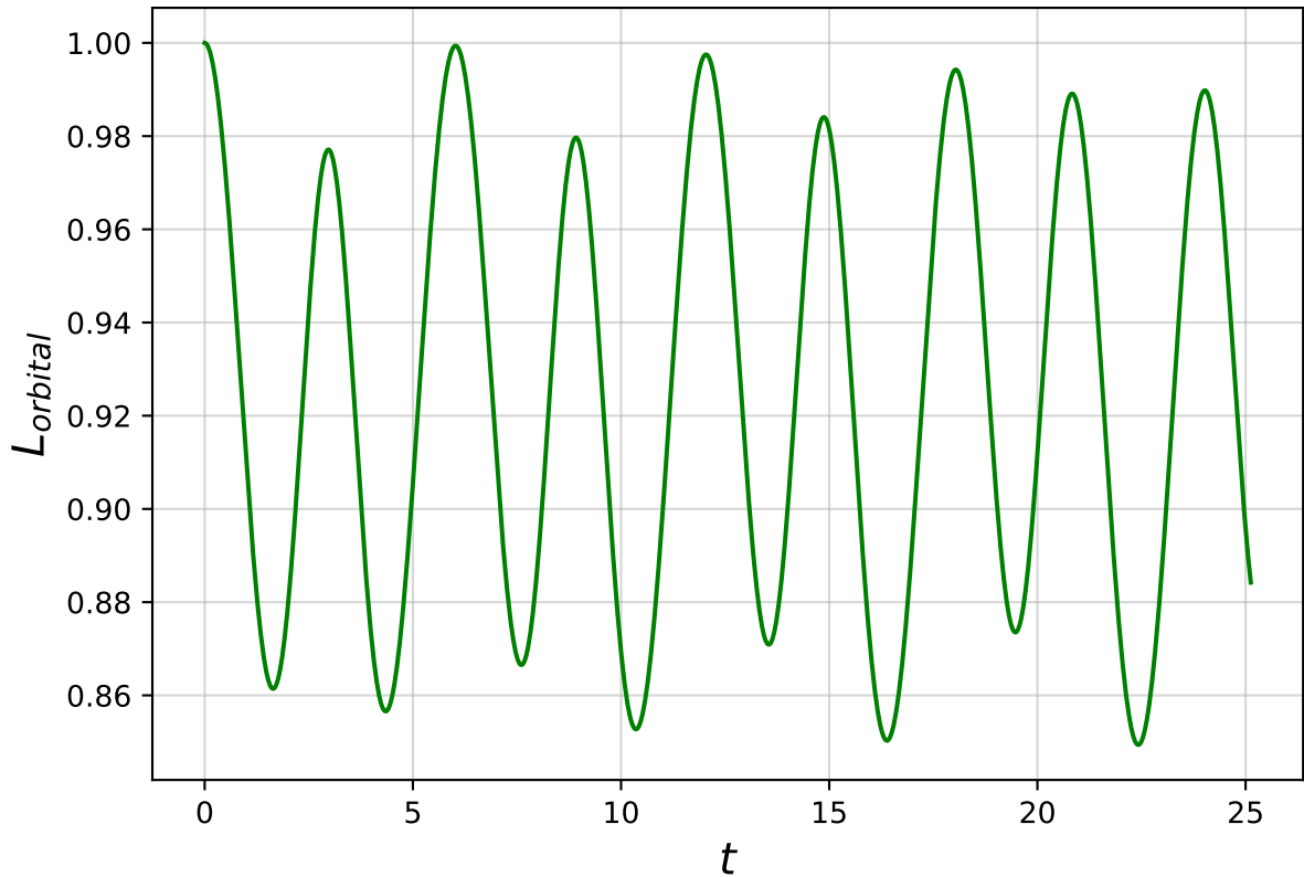
Orbital Angular Momentum vs. Time of M_1=1.0 , M_2=1\text{e-}20 Binary
