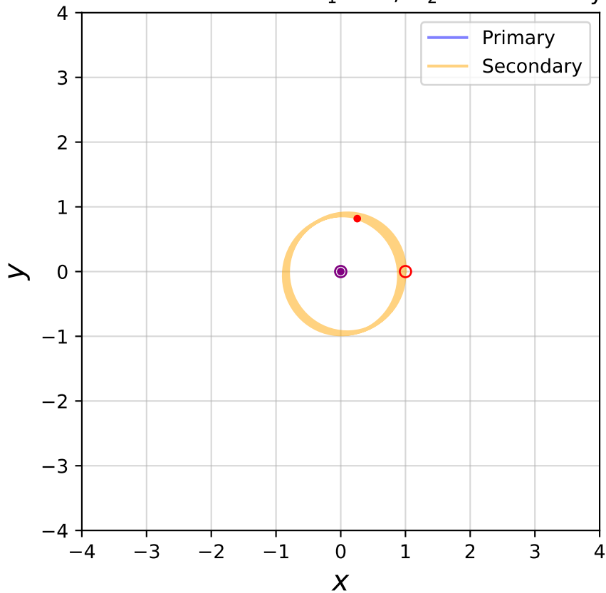
Position vs. Time of M_1=1.0 , M_2=1e-20 Binary
