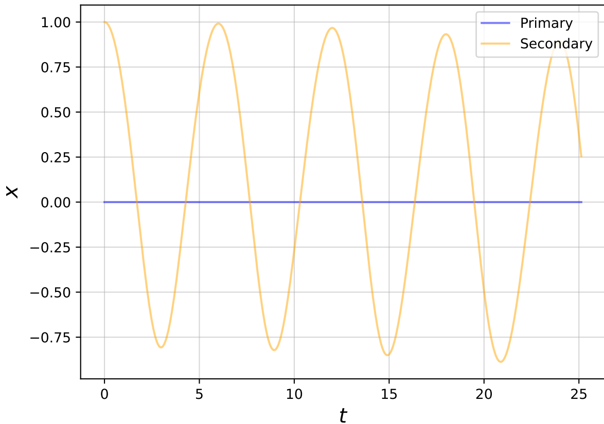
x Position vs. Time of M_1=1.0 , M_2=1e-20 Binary
