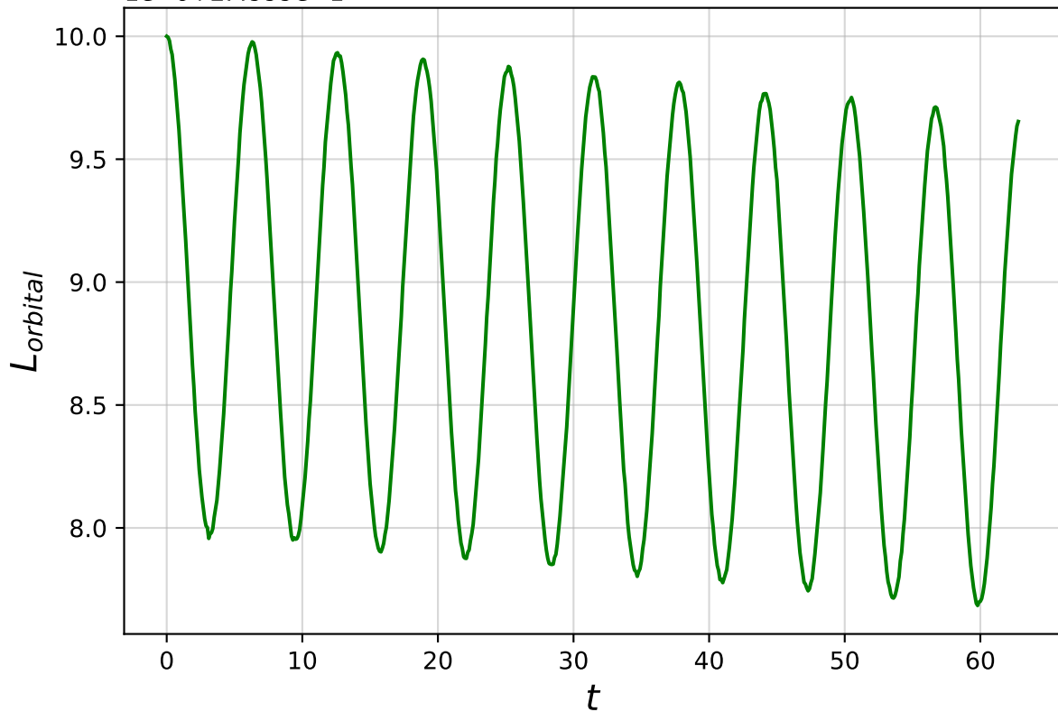
Orbital Angular Momentum vs. Time of M_1=0.5 , M_2=0.5 Binary 1e-6+2.4999e-1
