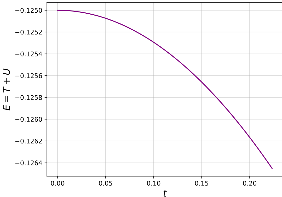
Energy vs. Time of M_1=0.5 , M_2=0.5 Binary
