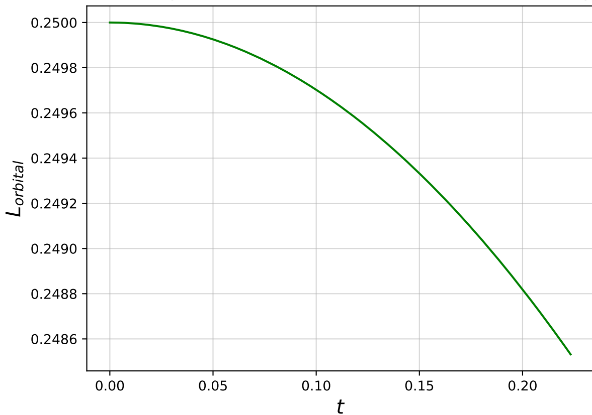
Orbital Angular Momentum vs. Time of M_1=0.5 , M_2=0.5 Binary
