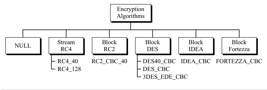
Figure 17.6 Encryption/decryption algorithms
