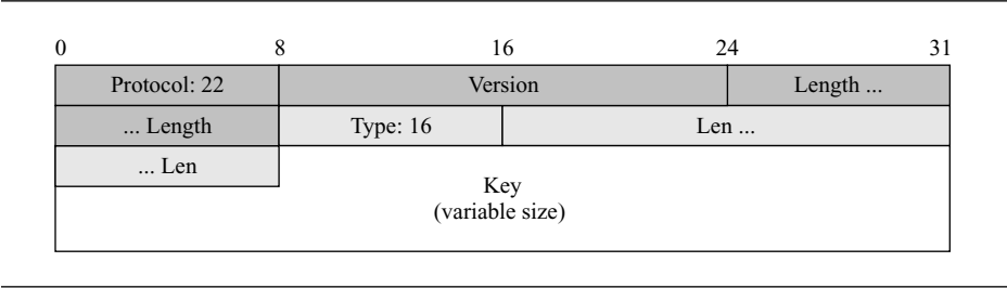
Figure 17.36 ClientKeyExchange message
