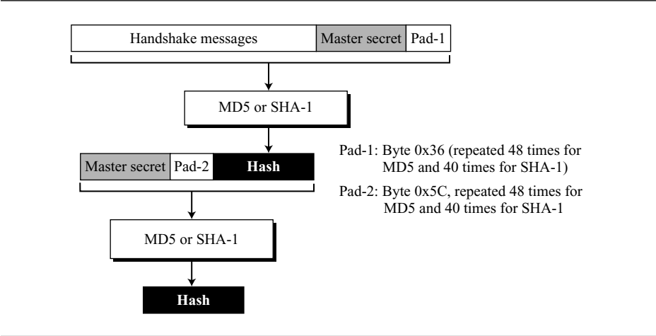
Figure 17.35 Hash calculation for CertificateVerify message
