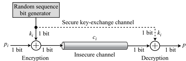
Figure 5.22 One-time pad
