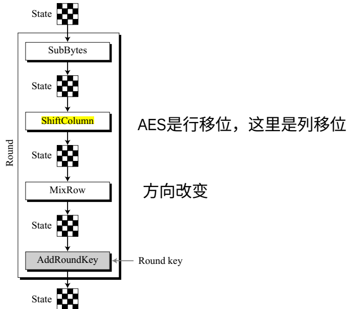
Figure 12.15 Structure of each round in the Whirlpool cipher
