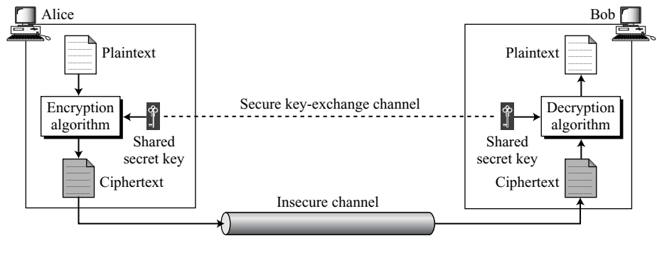
Figure 3.1 General idea of symmetric-key cipher
