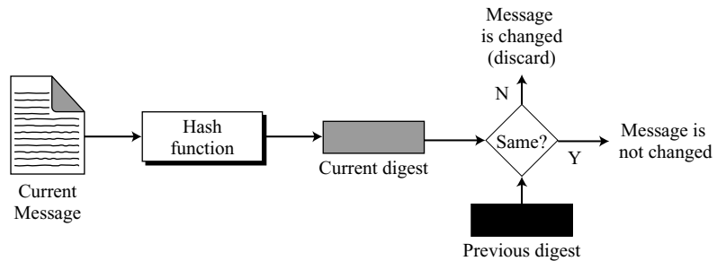
Figure 11.2 Checking integrity
