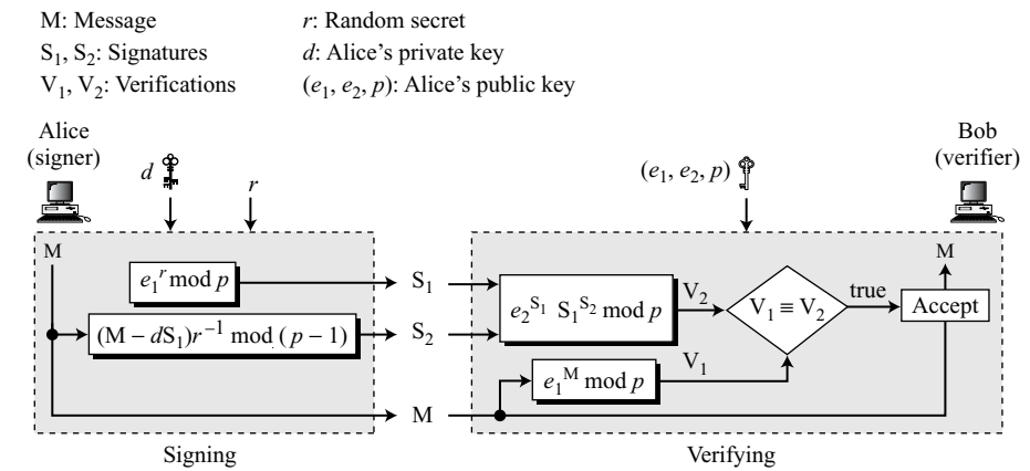
Figure 13.10 ElGamal digital signature scheme
