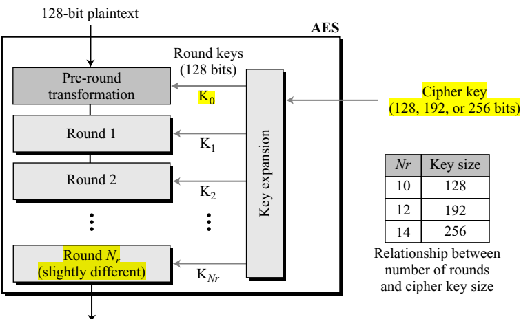
Figure 7.1 General design of AES encryption cipher
