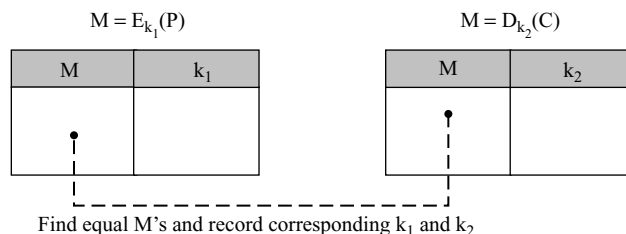
Figure 6.15 Tables for meet-in-the-middle attack
