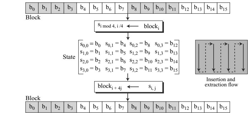
Figure 7.3 Block-to-state and state-to-block transformation
