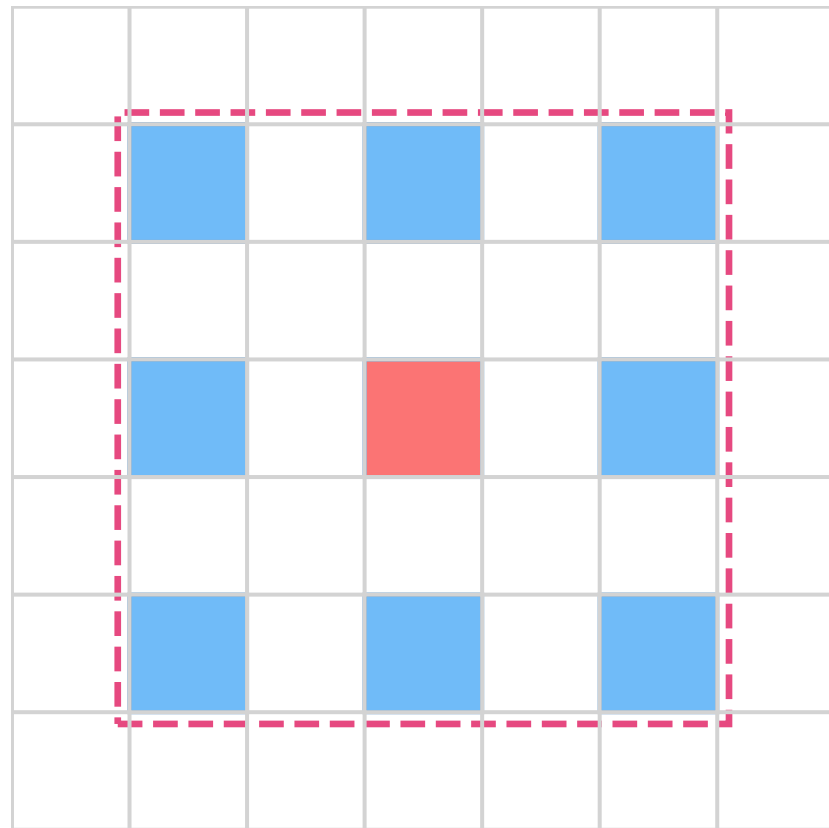
(b) 空洞卷积 (Dilation=2) 感受野: 5x5
