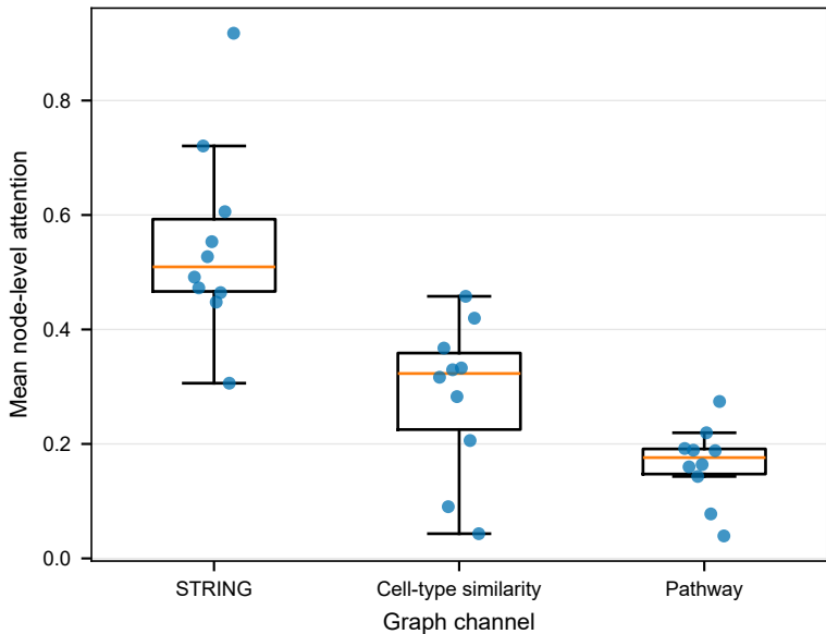
Attention stability across ensemble seeds
