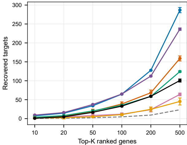
a Hidden target recovery
