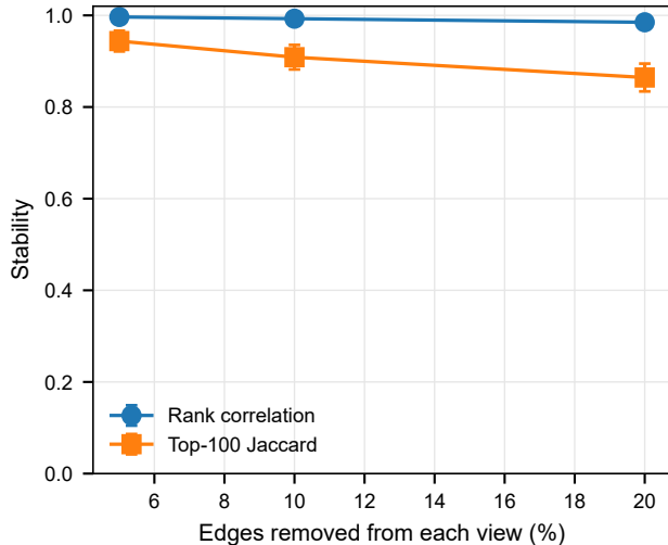
b Edge-dropout sensitivity
