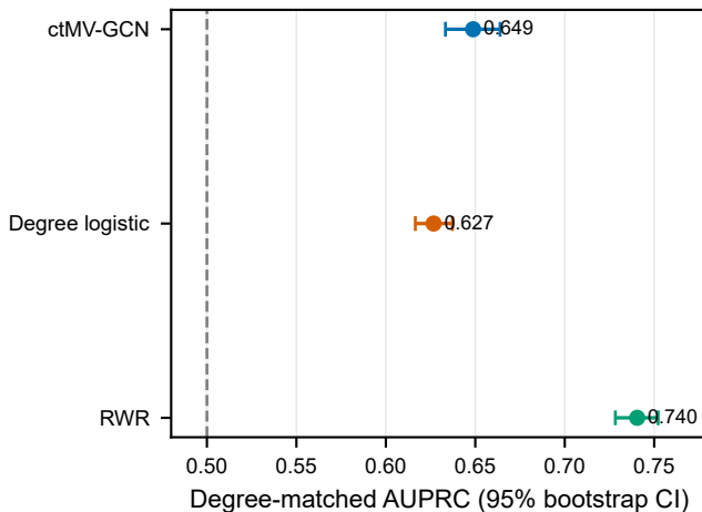
c Nonlinear degree residualization
