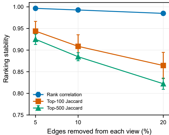
d Inference-time edge removal
