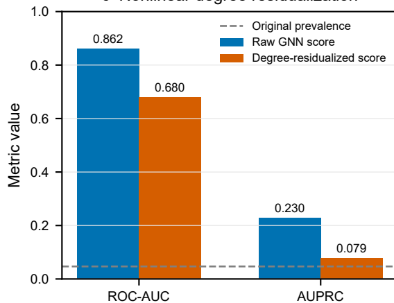
c Nonlinear degree residualization
