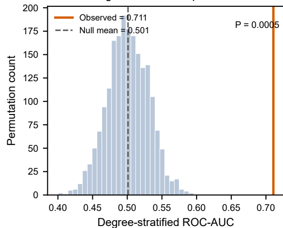
b Degree-conditional permutation
