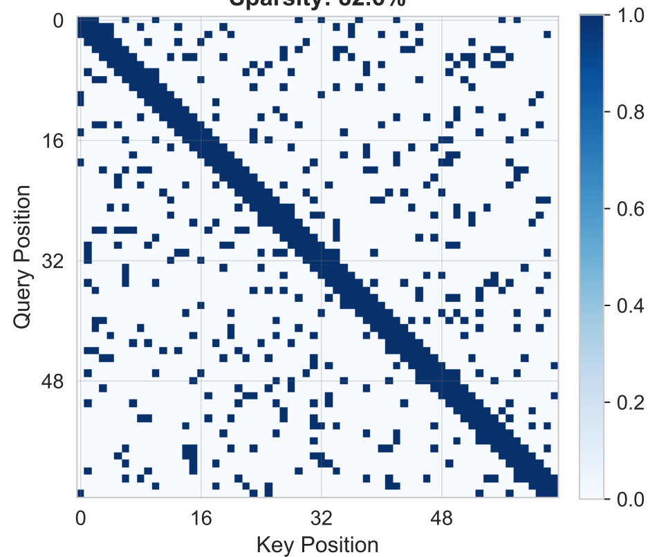
Random (10%) Sparsity: 82.6%
