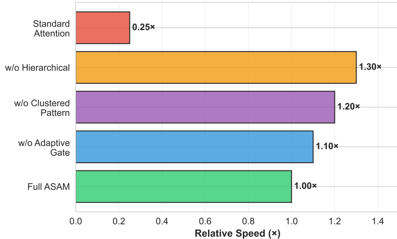
Ablation Study: Inference Speed
