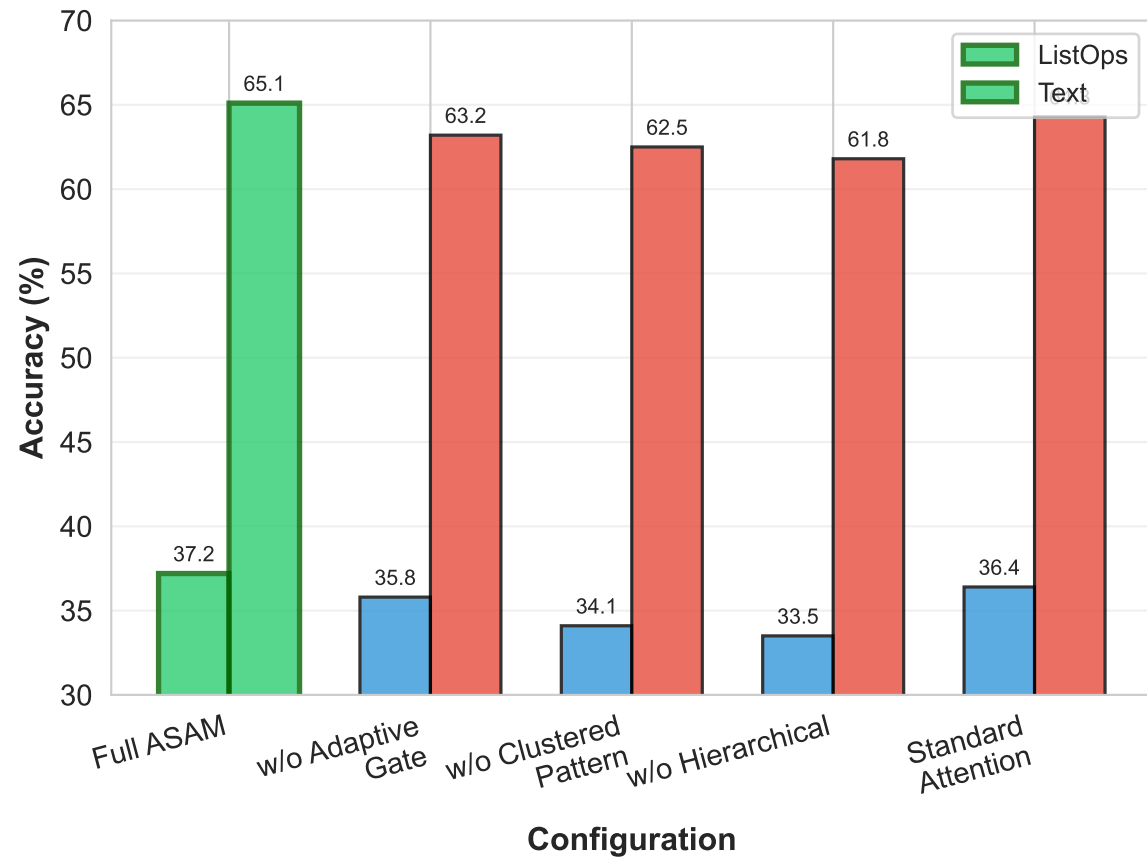
Ablation Study: Task Performance
