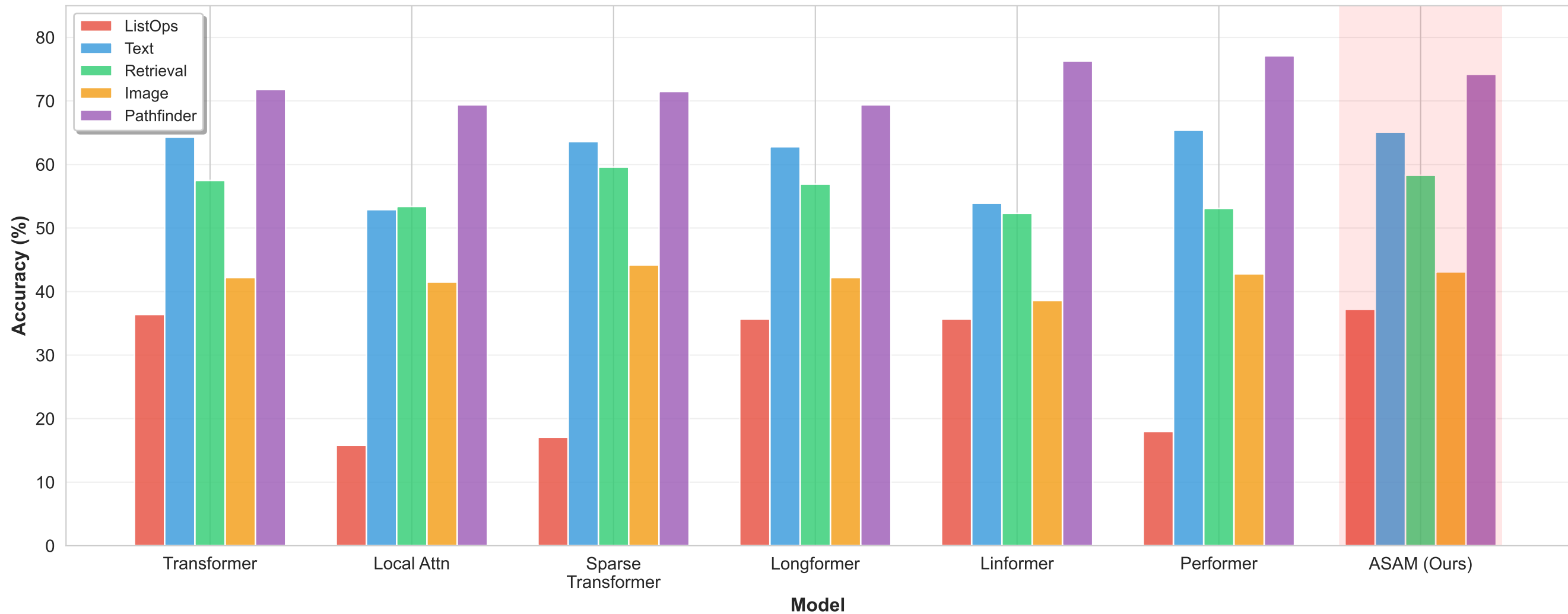
Long Range Arena (LRA) Benchmark Results
