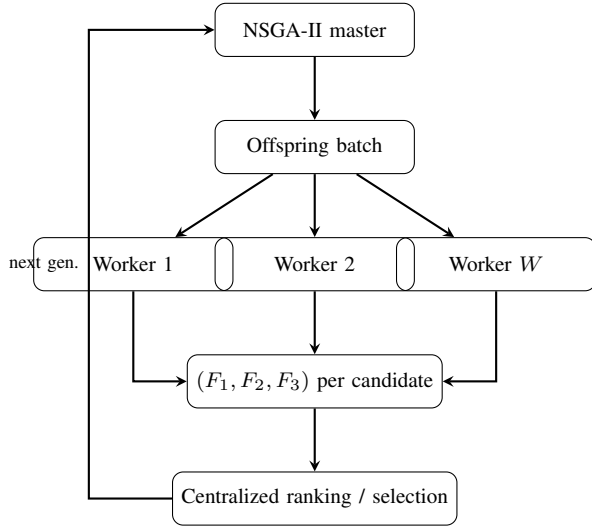
Fig. 2. Master-worker parallel framework. Only fitness evaluation is distributed; selection, crossover, mutation, RNG, archiving, and budget accounting stay centralized, preserving exact reproducibility.
