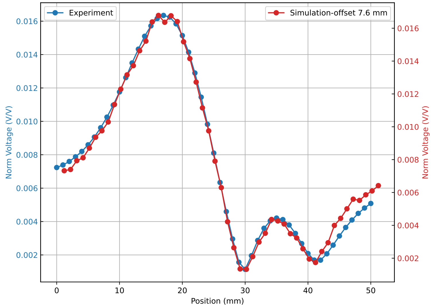
Alucoil - LVDT Validation
