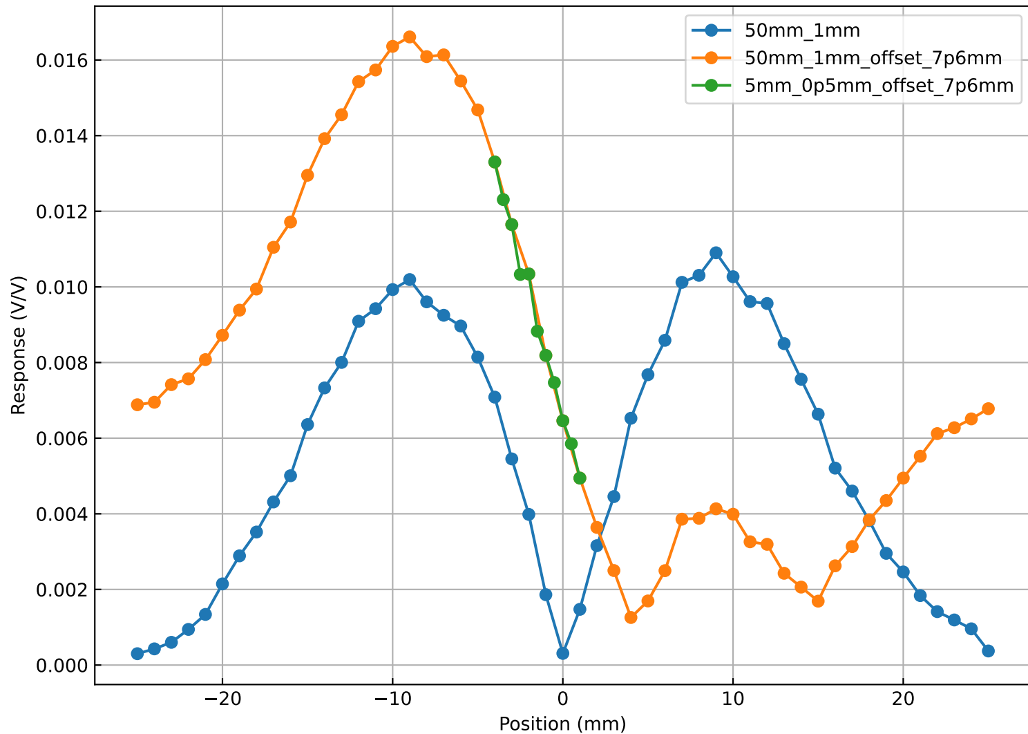
LVDT Response vs Position in Simulation
