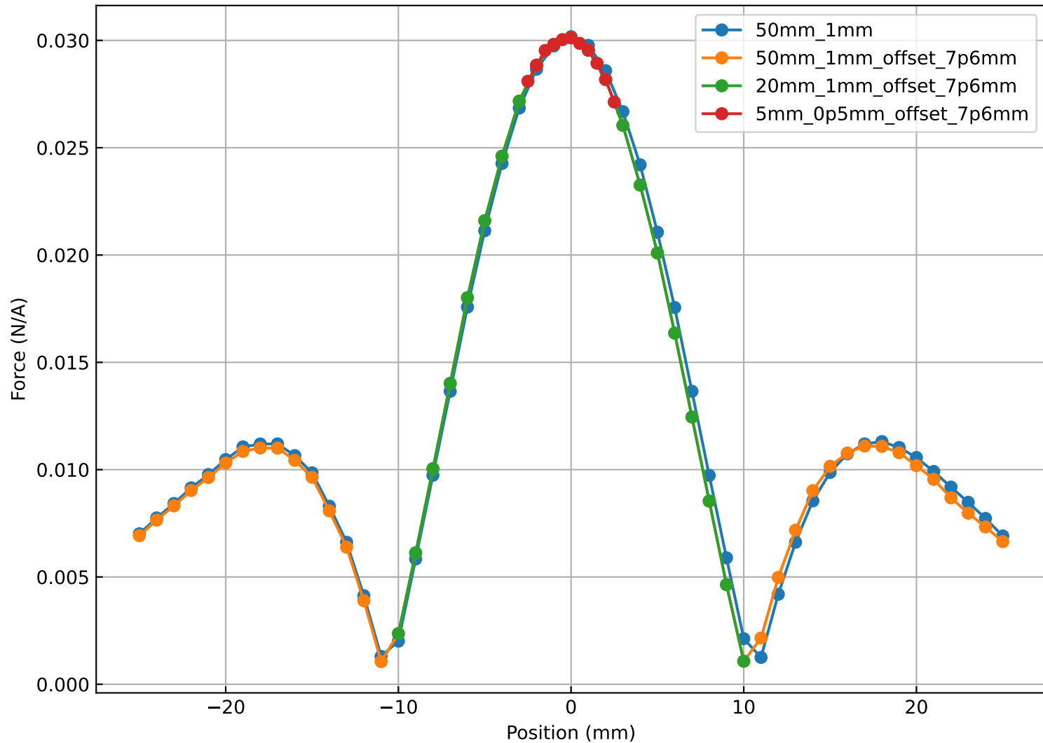
VC Force vs Position in Simulation
