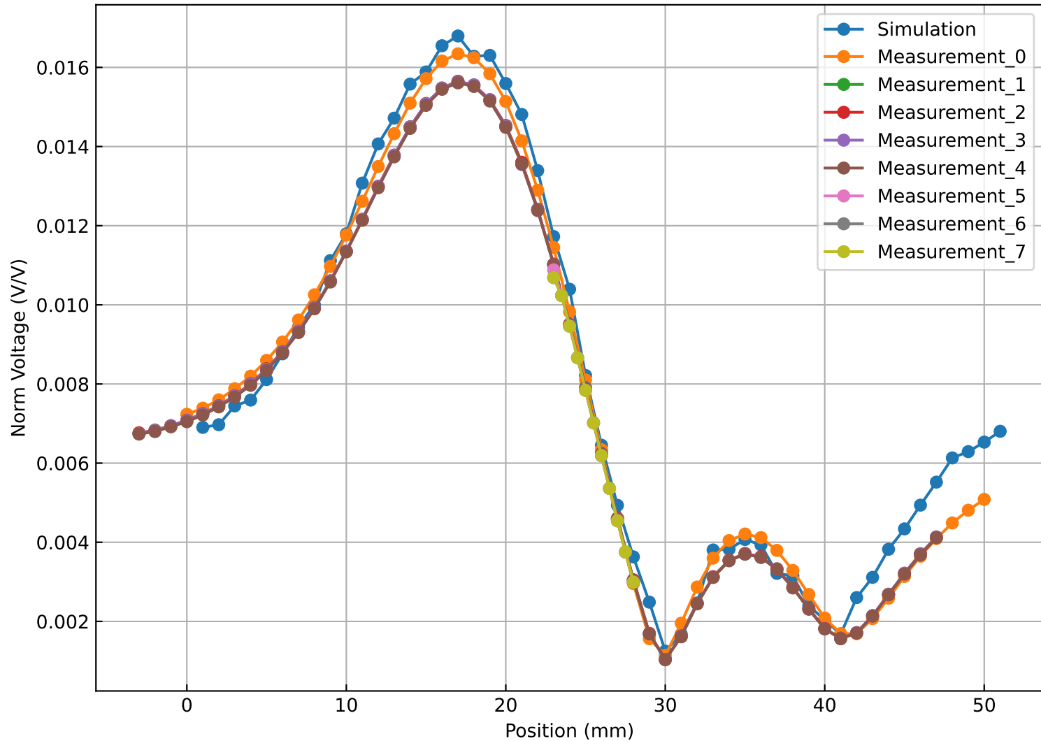
LVDT Response vs Position in Measurement
