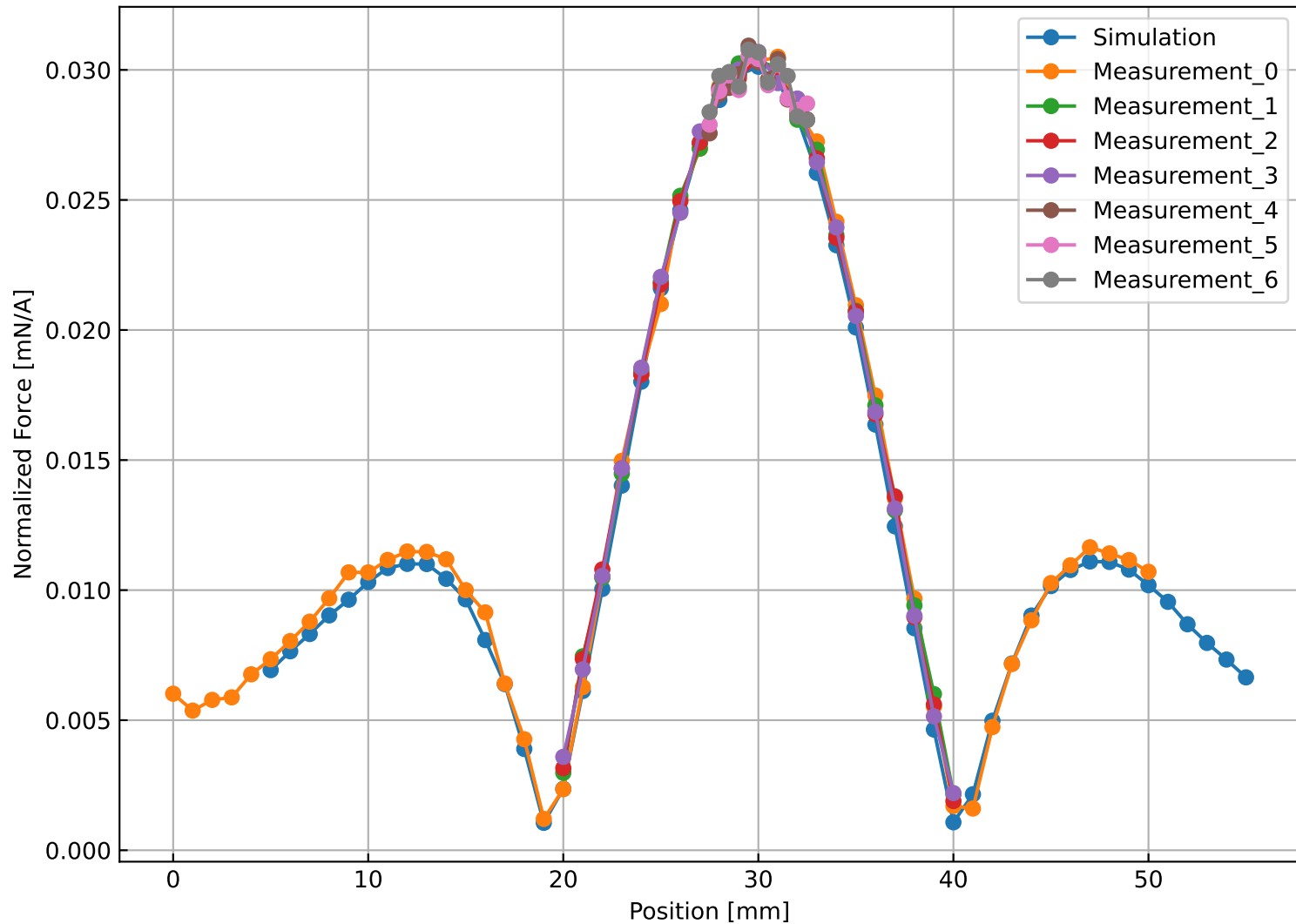
Alucoil - VC Force comparison
