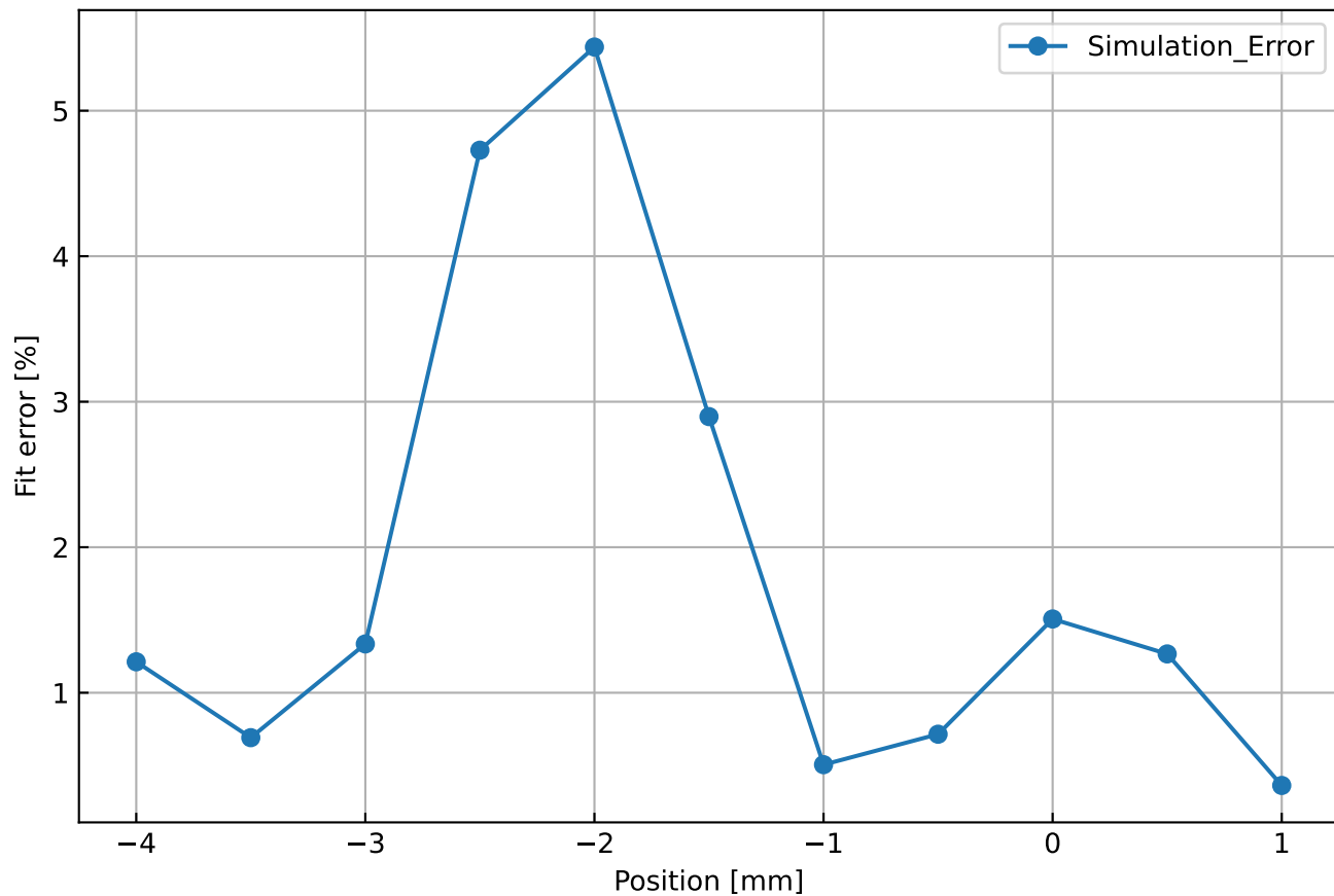
Alucoil - LVDT simulation
