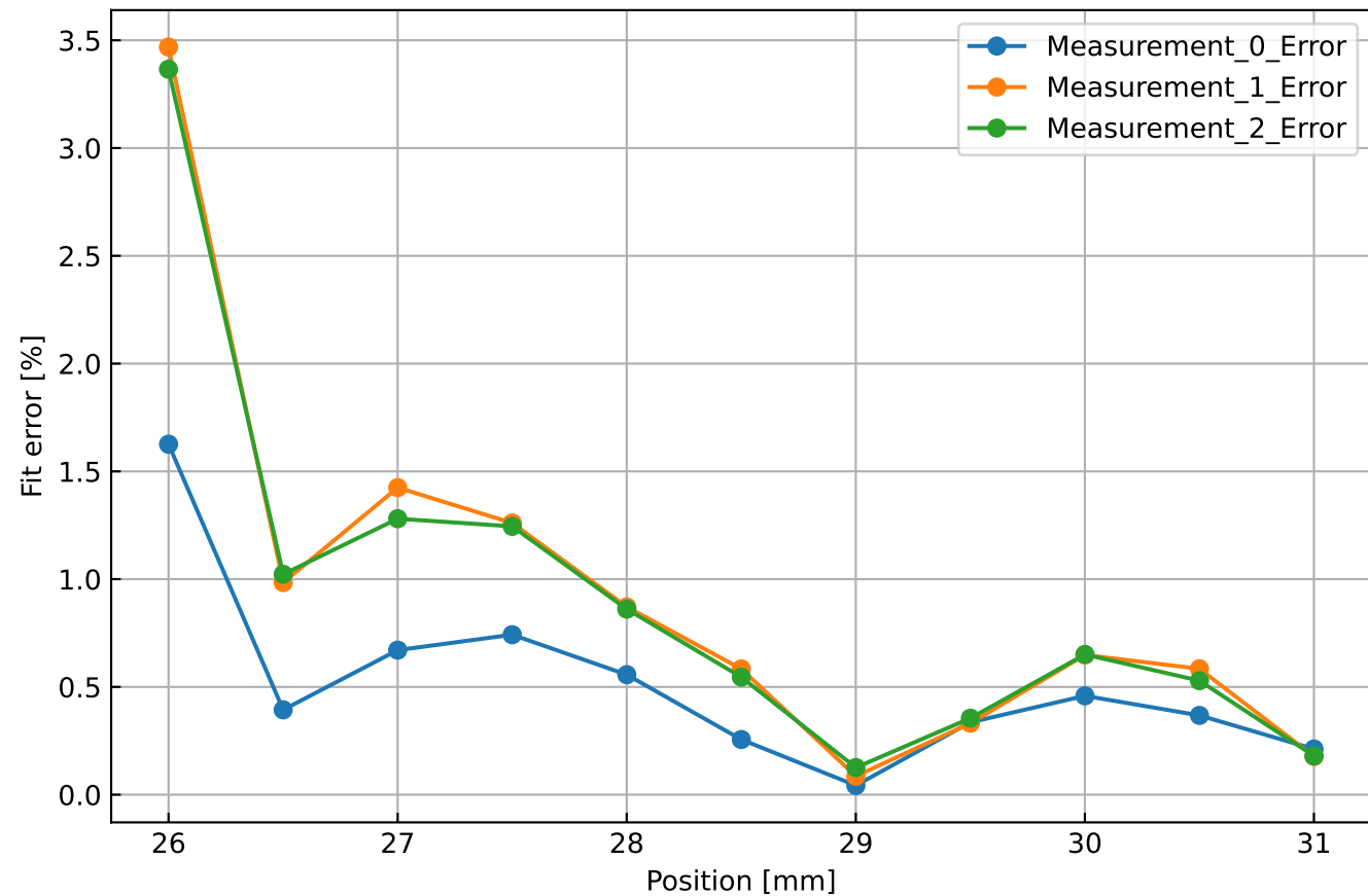
Alucoil - LVDT measurement
