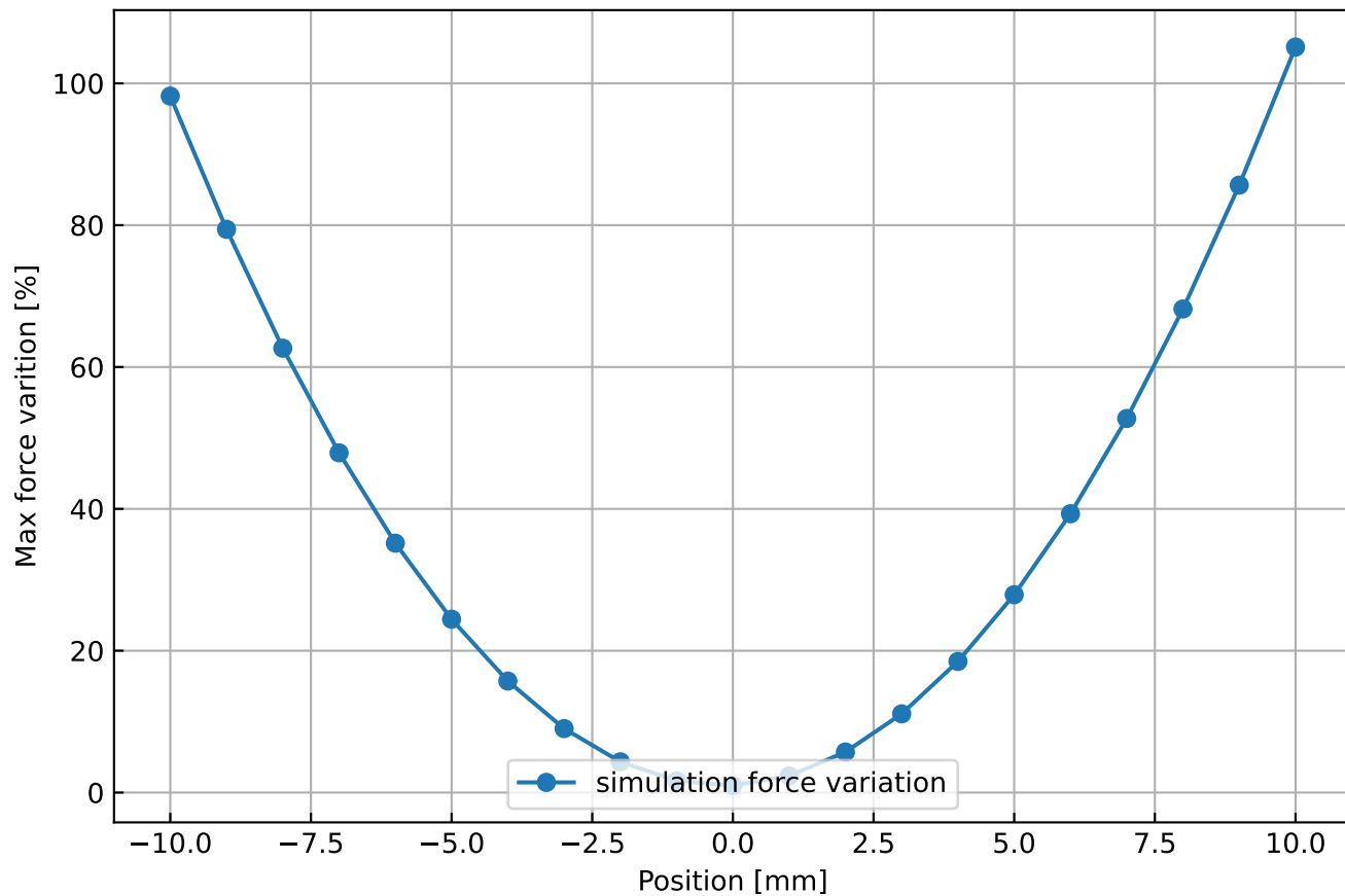
Alucoil - VC Force simulation
