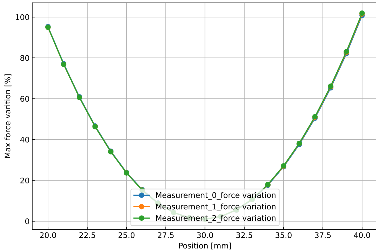
Alucoil - VC Force measurement
