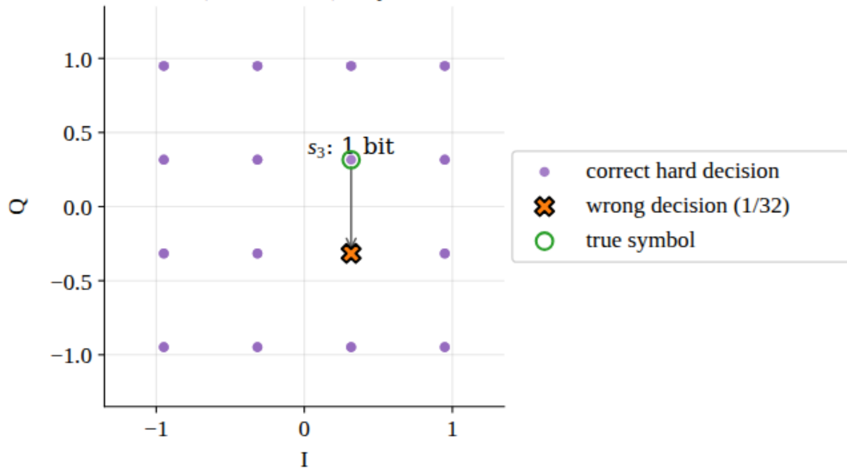
Reconstructed (EVM=34.7%), 1 symbol / 1 bit error
