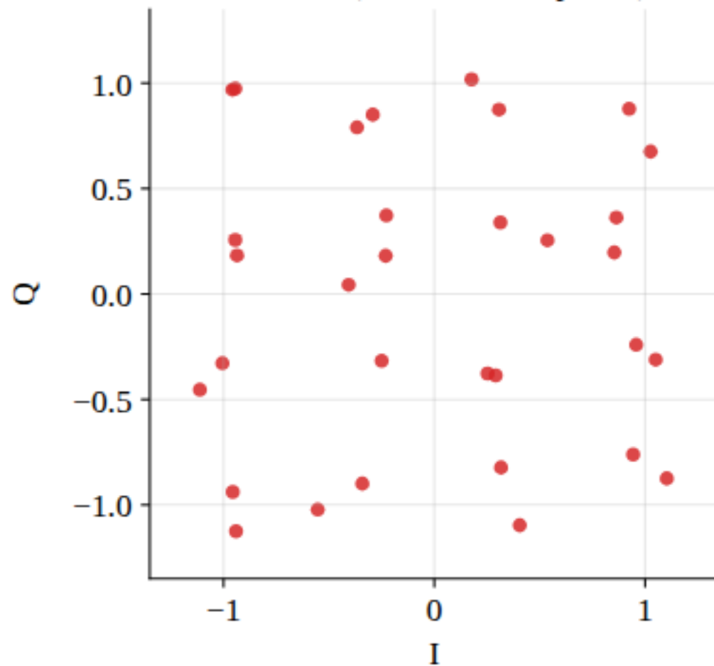
Received (EVM=15% impaired)
