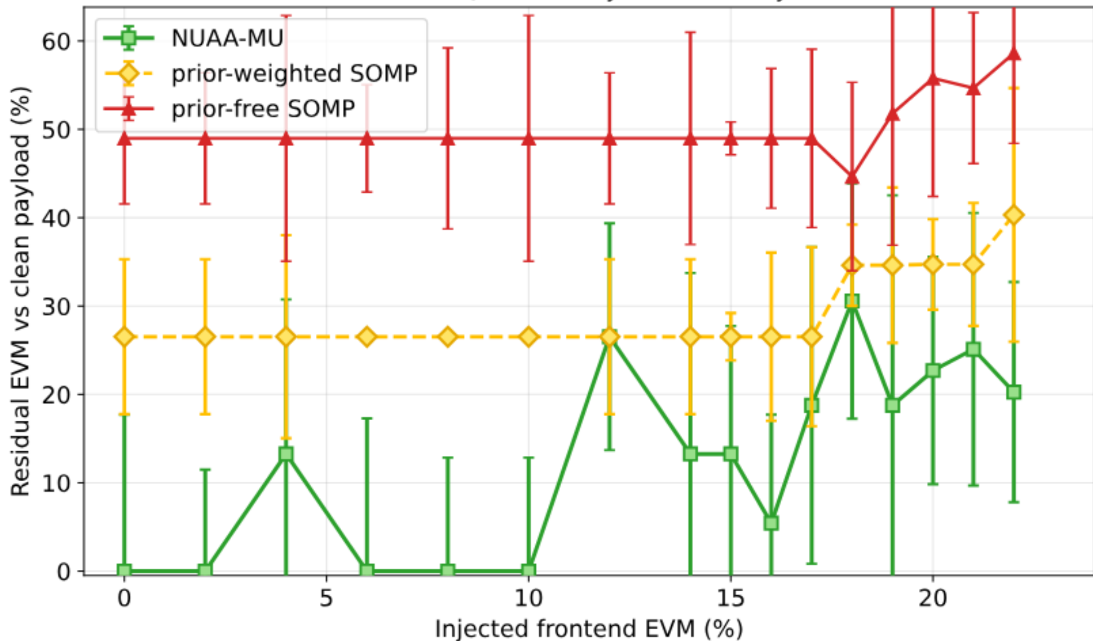
THz 16 QAM clean symbol recovery
