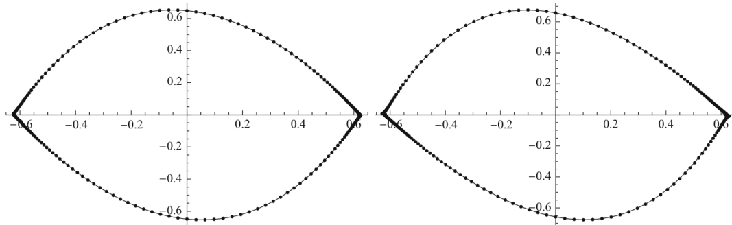
Figure 6: Heteroclinic orbits of the \Phi^6 -Van der Pol oscillator (102) for (a) \varepsilon = 2 and (b) \varepsilon = 4 . Solid: Runge-Kutta. Dashed: GPLP. Both orbit branches connecting the saddle points are accurately captured.
