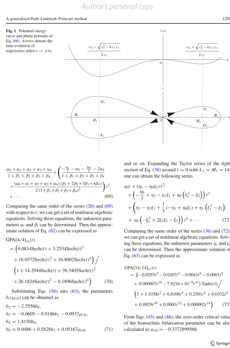
Figure 1: Potential energy curve and phase portraits for the Helmholtz–Duffing oscillator.
