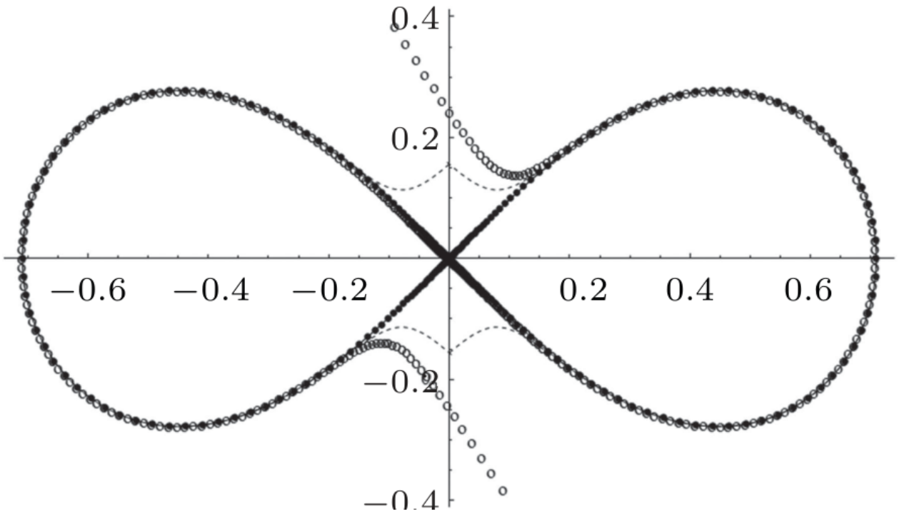
Figure 3: Figure 3. (Original Fig. 4) Homoclinic orbits of the Duffing-harmonic oscillator ( \lambda = -1, \mu = 5, \nu = 5 ). Solid: Runge-Kutta. Dotted: GPA[3/3].
